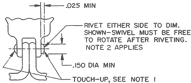
VIEW A-A SCALE 2/1
