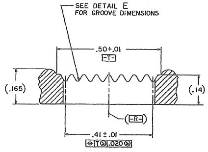
DETAIL F ROTATED 90° CCW SCALE: 10/1
