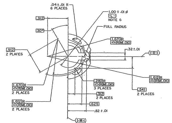
VIEW N-N
