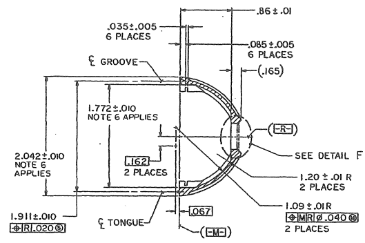
SECTION C-C NOTE 6
